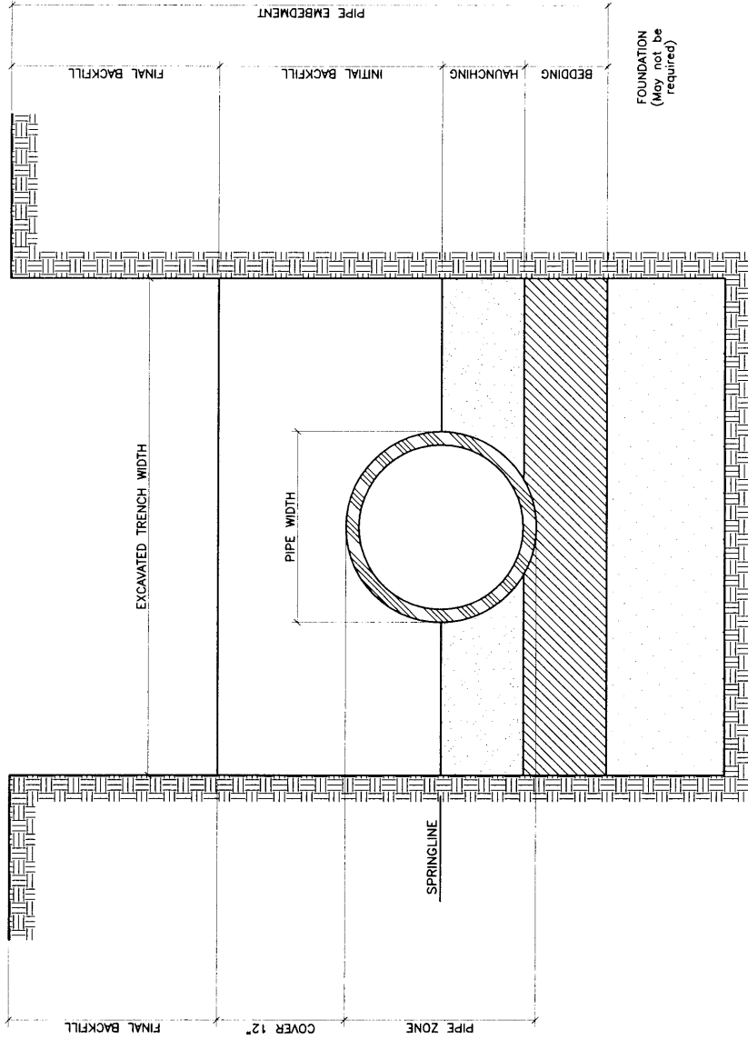
TRENCH CROSS-SECTION SHOWING TERMINOLOGY
