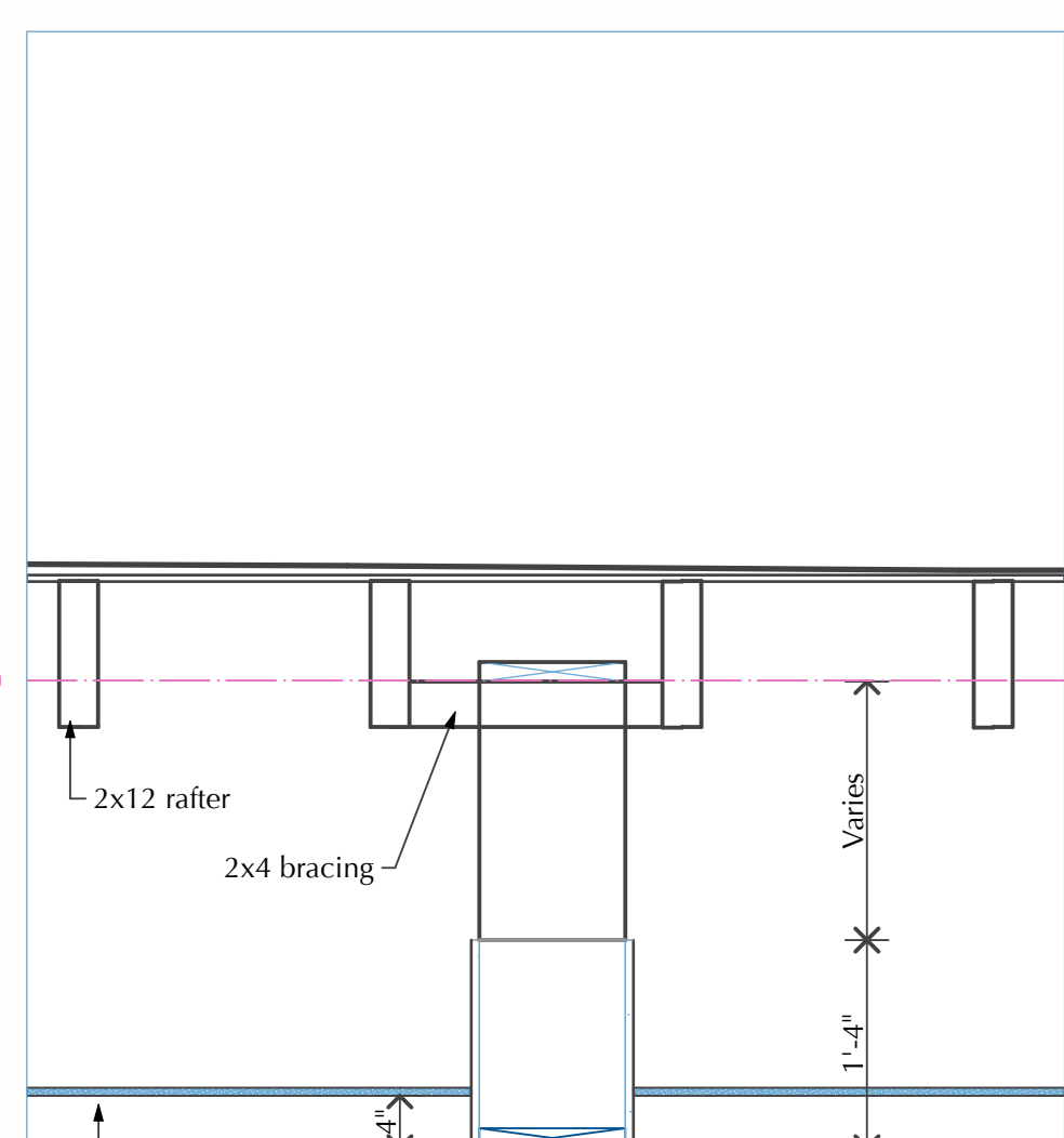
B Overflow Scupper Detail Scale: 3" = 1'-0"
