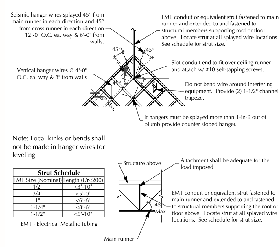
S Ceiling Brace Not To Scale
